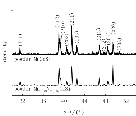
图1 \text{Mn}_{0.98}\text{Ni}_{0.02}\text{CoSi} 合金粉末样品的室温 XRD 图谱
