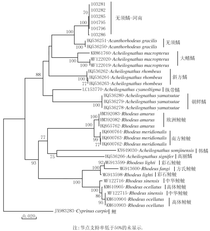
图2 基于线粒体COI基因构建的鳊属鱼类邻接法(neighbor-joining method, NJ)系统发育关系 Fig.2 Phylogenetic relationships of Acheilognathus based on neighbor joining method (NJ) constructed by mitochondrial COI gene
